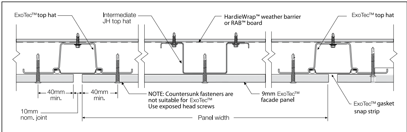
TOP HAT AND PANEL FIXING DETAIL FOR EXOTEC™ PANELS
