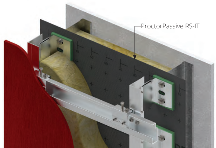
04/TUF-S-Xxxx-A4 TUF-S fixing A4 stainless steel
