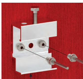
03/NV3-TUF-S-ADJ-3.5-M6 NV3 levelling hanger for TUF including adjust screw
