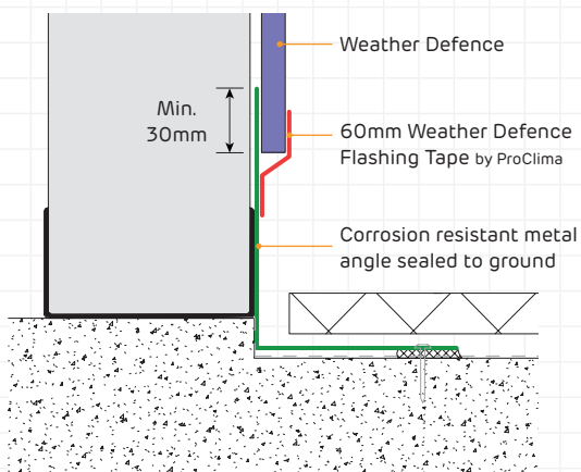
Figure 17 Wall base detail - Balcony
