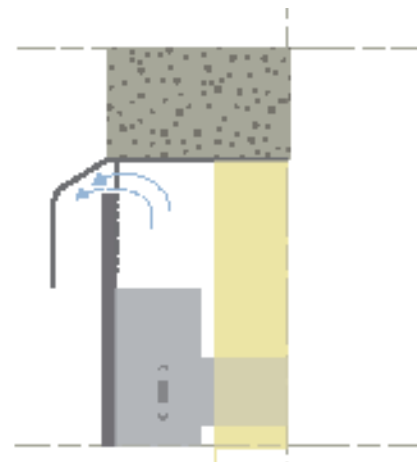
Figure 22: EQUITONE to render top abutment
