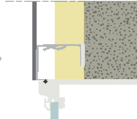
Figure 17: Flush Window/Jamb
