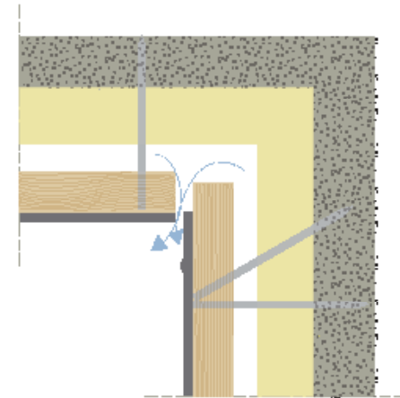
Figure 20: Soffit Detail
